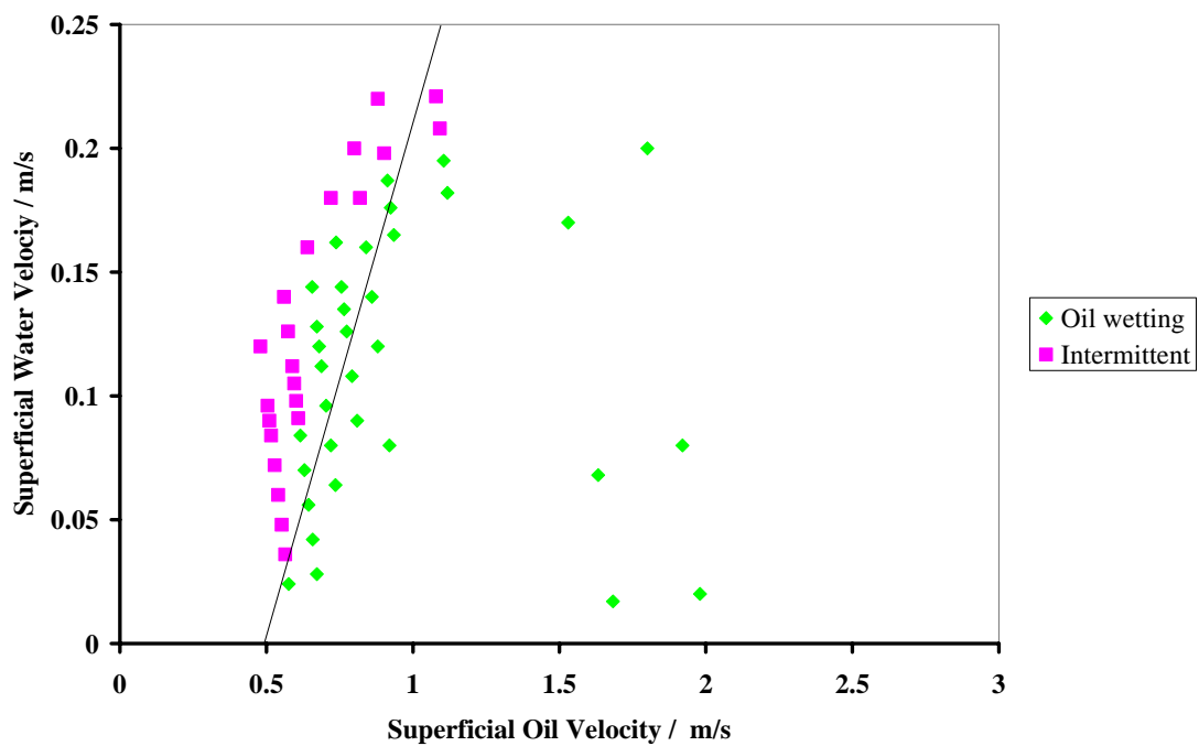
FIGURE 12 - Phase wetting map for AXL at different superficial oil and water velocities in the 5 degree upward inclined oil-water two-phase flow
